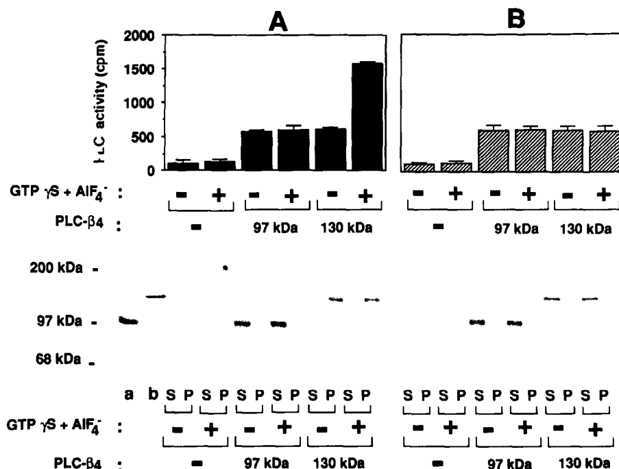
Fig. 4. Reconstitution of purified PLC- \beta 4 with the membrane fraction of C 6 Bu-1 rat glioma cells. Each purified PLC- \beta 4 was incubated with the membrane fractions prepared by washing with the buffers containing 0 M (A) or 2 M KCl (B) for 30 min and half of the incubation mixture was used for the measurement of inositol phosphates (upper panels) while the other half was for immunoblot after resolving into supernatant (lane, S) and precipitate (lane, P) by centrifugation. Lane: a, the purified 97 kDa PLC- \beta 4; b, the purified 130 kDa PLC- \beta 4
